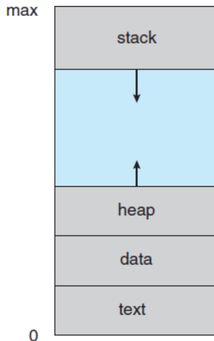
Process in Memory
