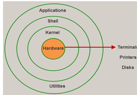
Architecture of Linux
