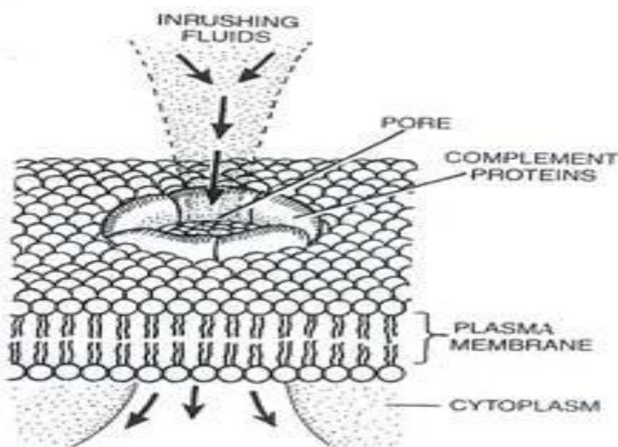
Fig. 8.7. Complement proteins creating a hole in the plasma membrane.
