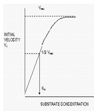
Fig. 3.6. A plot of V_0 vs. substrate concentration S .
