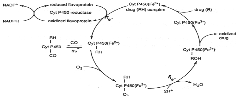
Fig: Cyt P450 catalysed hydroxylase cycle
