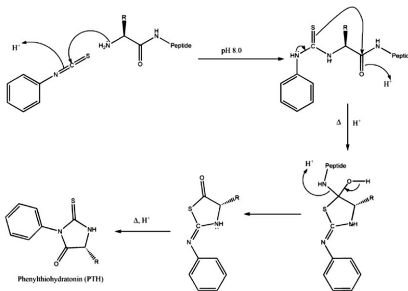
Edman Degradation with generic amino acid peptide chain.
