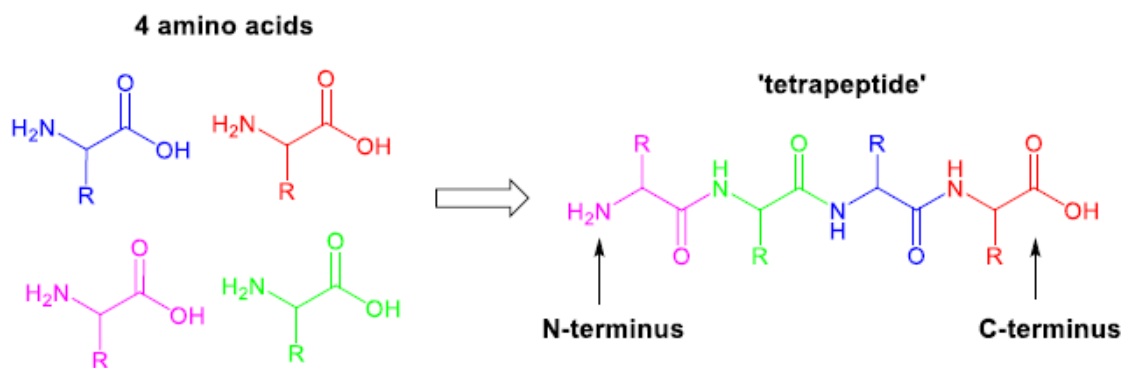
General structure of a peptide containing four amino acids
