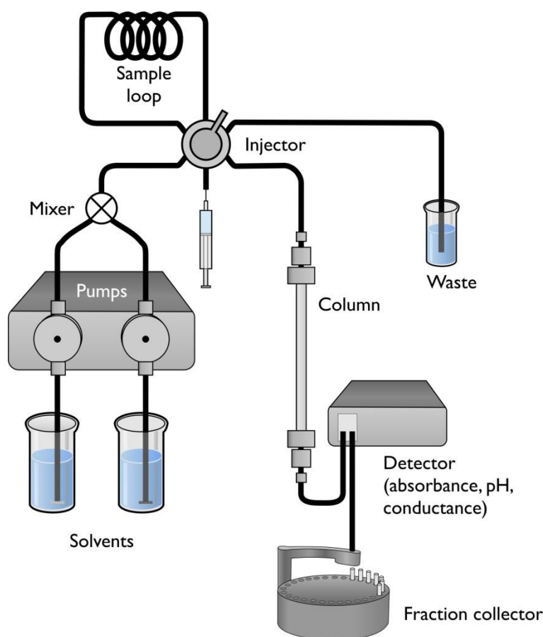
Figure Schematic layout diagram of the HPLC equipment. The system consists of pumps that ensure the high-pressure delivery of a two-component mobile phase, a mixing unit, a sample injector, a chromatographic column and a detector.
