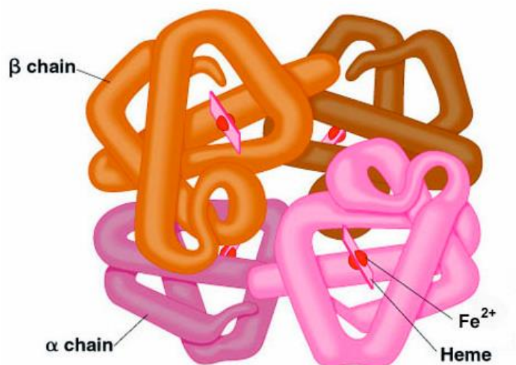
Structure of Hemoglobin
