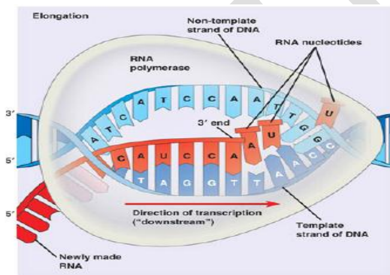
Transcription elongation
