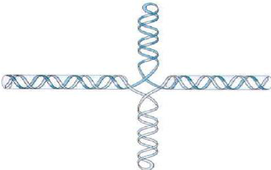
Cruciform DNA
