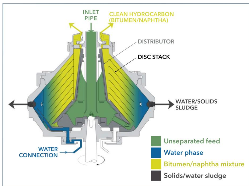
Disc centrifuge
