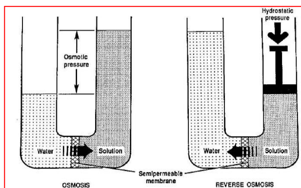
Reverse osmosis
