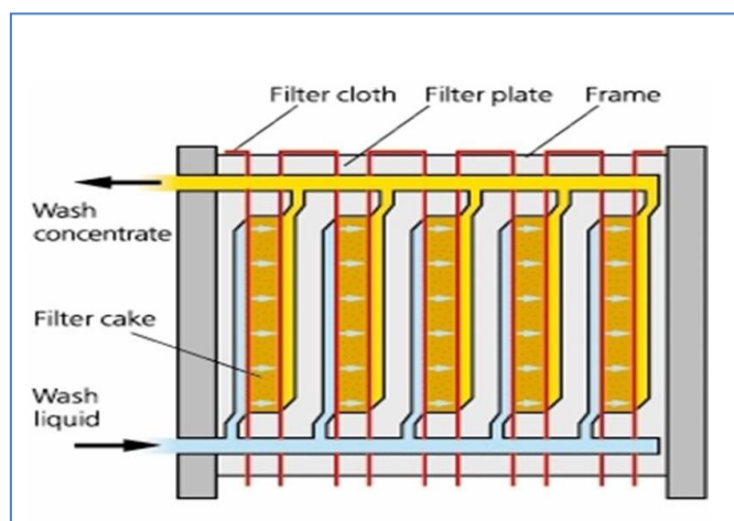
Plate and frame filters
