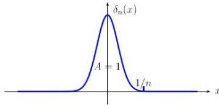
Figure 4.7: The Dirac function \delta_n(x) .
