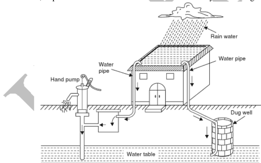
Roof-top rainwater harvesting by recharging (i) through hand pump or (ii) through abandoned dugwell.
