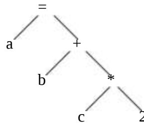
Figure 1.8: Syntax Tree
