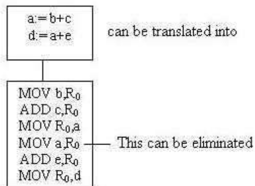
Figure 4.2:Instruction selection
