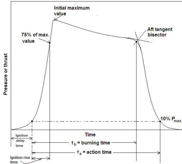
Fig. Definition of burning time and action time
