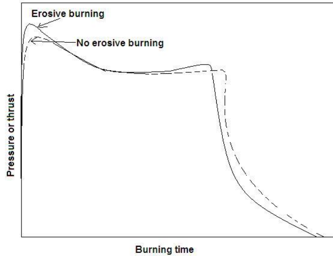
Fig. Typical pressure-time curve with and without erosive burning
