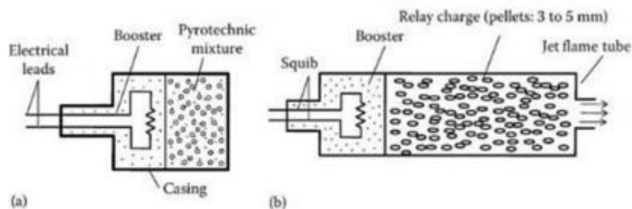
!6 Schematic of pyrotechnic igniters: (a) basket igniter; (b) jet flame pyrotechnic igniter.
