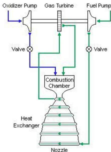
Fig. 1.10 - EXPANDER
