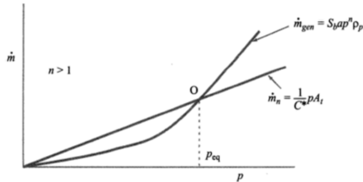
Fig. 5.13 Unstable Operation for n > 1
