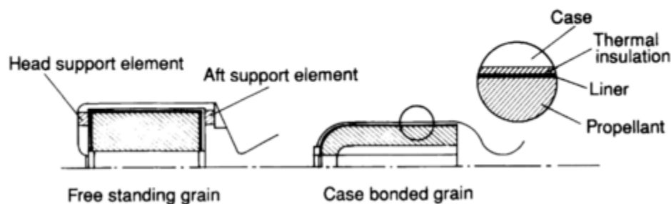
FIG. 2.1. Case bonded grain.
