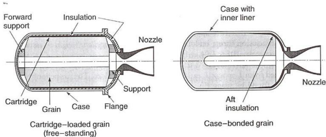
FIGURE 11-14. Simplified schematic diagrams of a free-standing (or cartridge-loaded) and a case-bonded grain.
