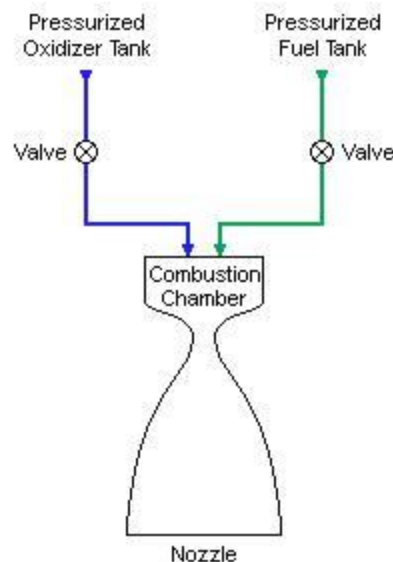
Fig. 1.11 - PRESSURE-FED
