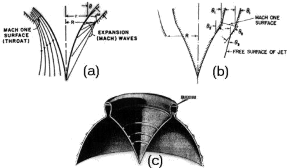
Comparison of spike nozzles with (a) external expansion, (b) internal-external expansion, and (c) internal expansion [from Berman and Crimp, 1961]
