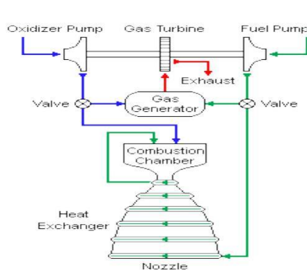
Fig. 1.8 - GAS GENERATOR
