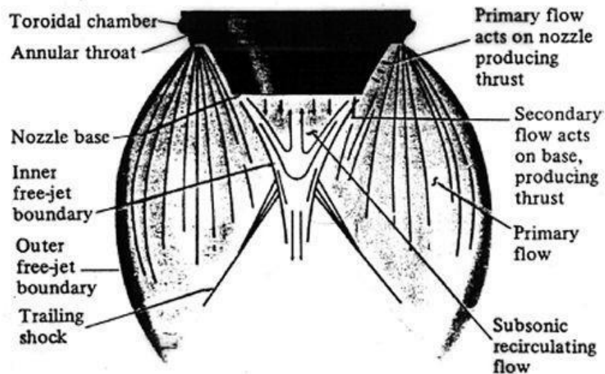
Example of an aerospike nozzle with a subsonic, recirculating flow [from Hill and Peterson, 1992]
