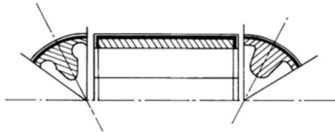
FIG. 2.6. Wagon wheel configuration.
