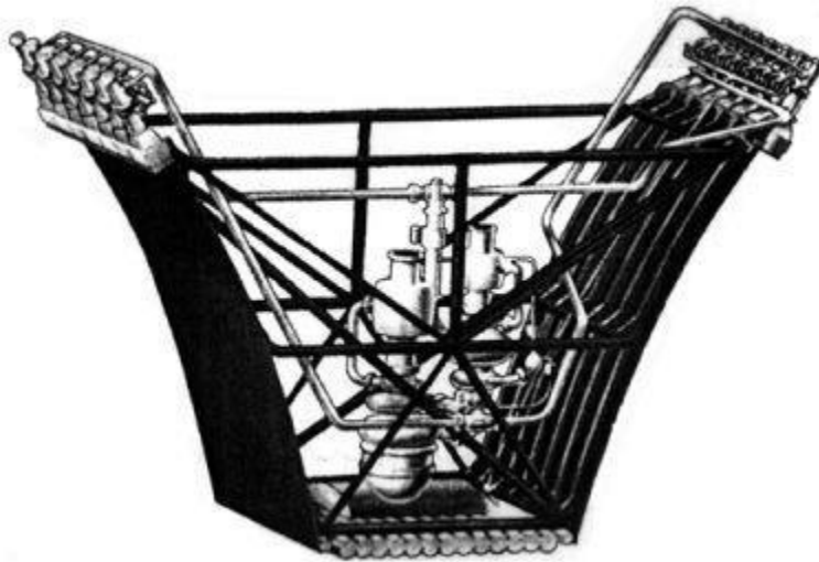
Rocketdyne RS-2200 linear aerospike engine [from Flinn, 1996]
