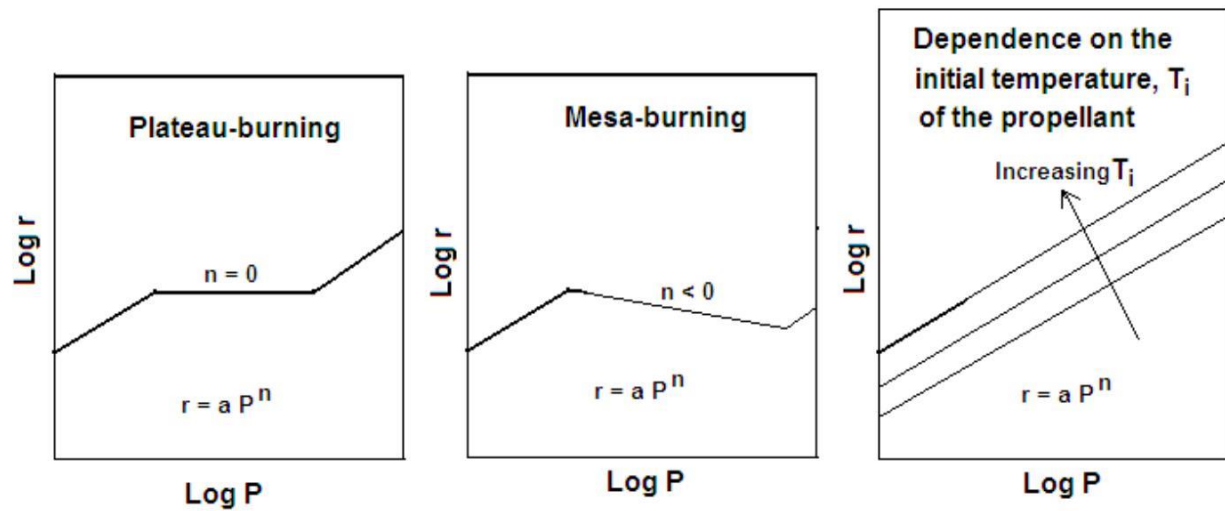
Fig. Burning rate versus pressure
