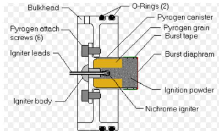
Comparison between Pyrotechnic and Pyrogen Igniters
