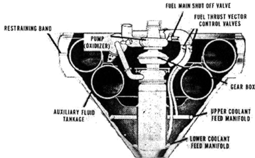
Example of a truncated, conical spike [from Berman and Crimp, 1961]
