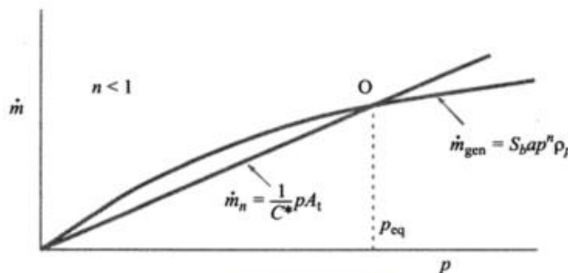
Fig. 5.14 Stable Operation for n < 1
