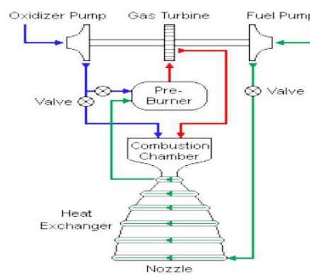
Fig. 1.9 - STAGED COMBUSTION
