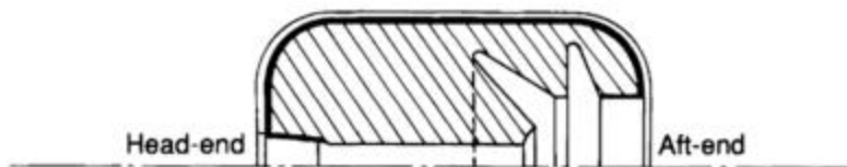
FIG. 2.4. Conocyl configuration.
