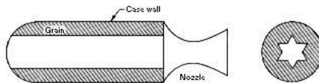
Fig.1-Schematic of solid-propellant rocket
