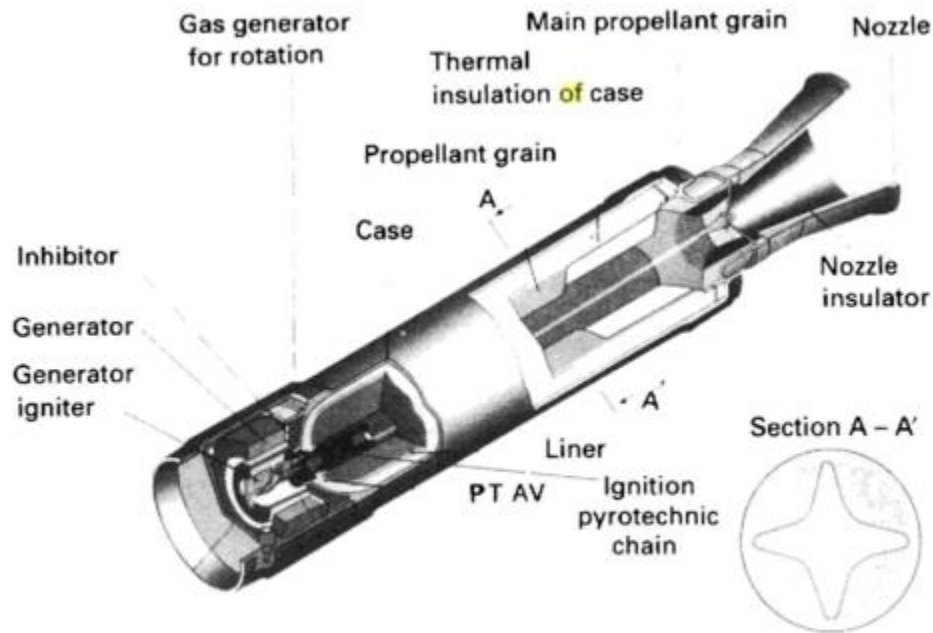
FIG. 1.1. Typical rocket motor.
