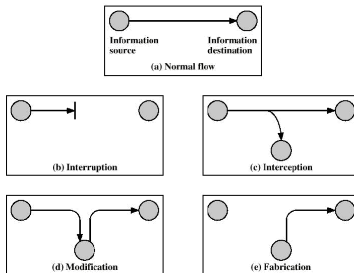
Figure 1.1 Security Threats
