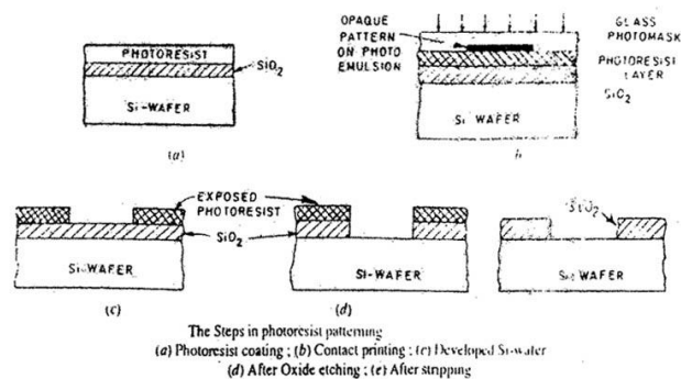
Photolithographic Process Steps
