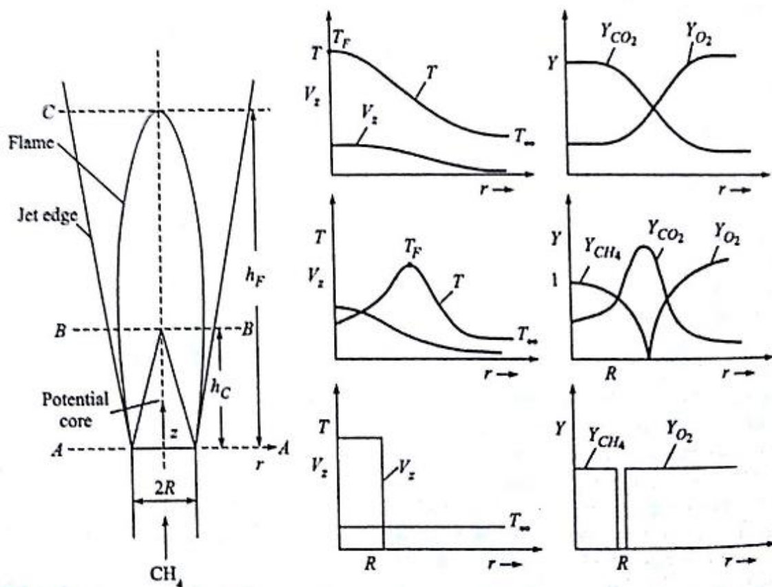
The flame structures of laminar gaseous jet diffusion flame.
