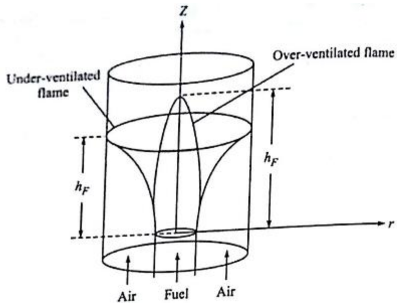
Types of diffusion flame shape: (a) over-ventilated, and (b) under-ventilated.
