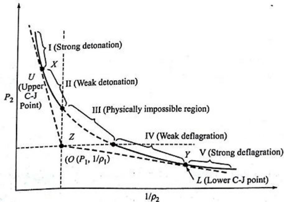
Figure 5.2 Hugoniot curve with various regimes.
