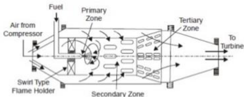
Combustion Chamber with Downstream Injection and Swirl Holder
