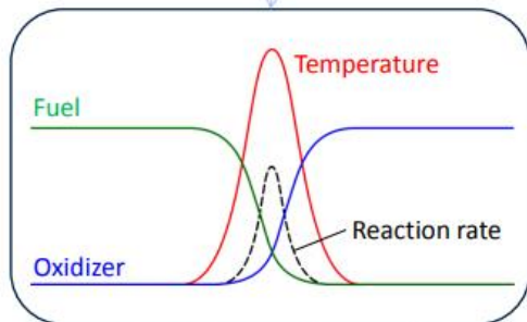
Structure of a diffusion flame (schematic)
