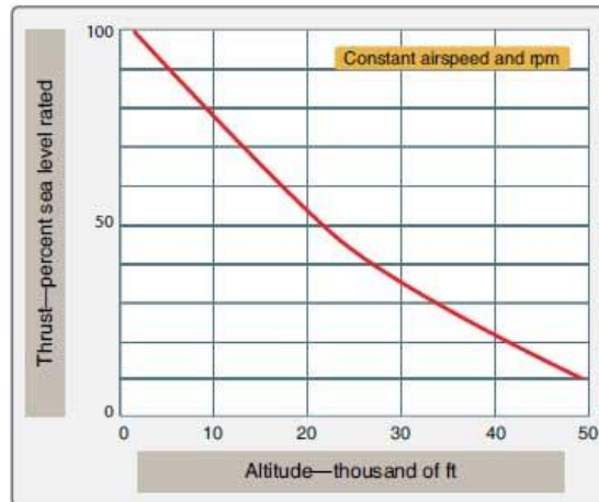
fig. 5. Effect of altitude on thrust output.
