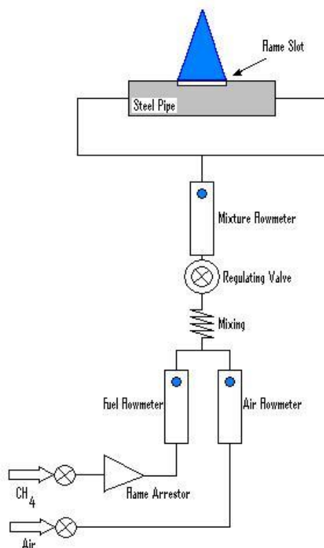
Figure 3: Design of Slot Burner Apparatus
