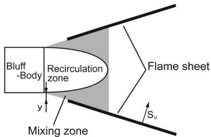
Figure 8.31 Flame stabilization by recirculation
