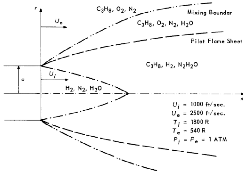
Schematic of ignition of propane-air mixture with hydrogen-air pilot.
