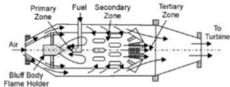
Combustion Chamber with Upstream Injection with Bluff-body Flame Holder.
