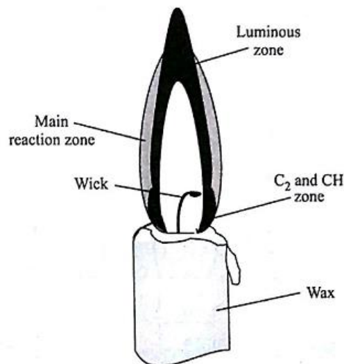
Reaction zones in a candle flame.
