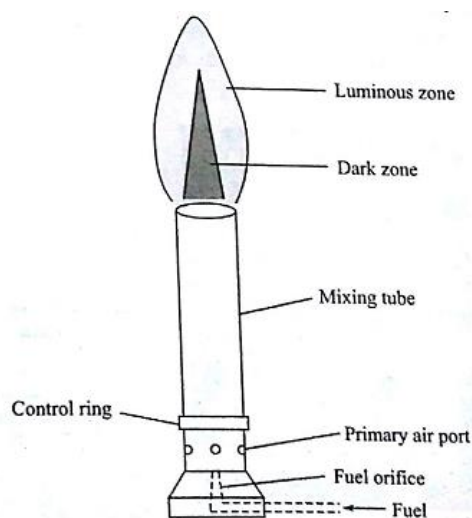
Schematic diagram of a typical Bunsen burner (premixed burner).
