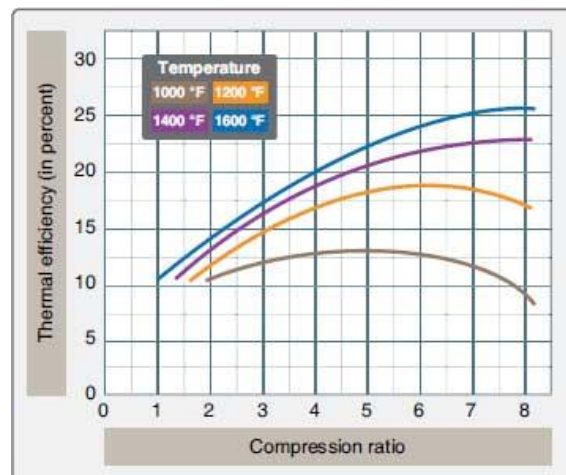
Fig.1. The effect of compression ratio on thermal efficiency.
