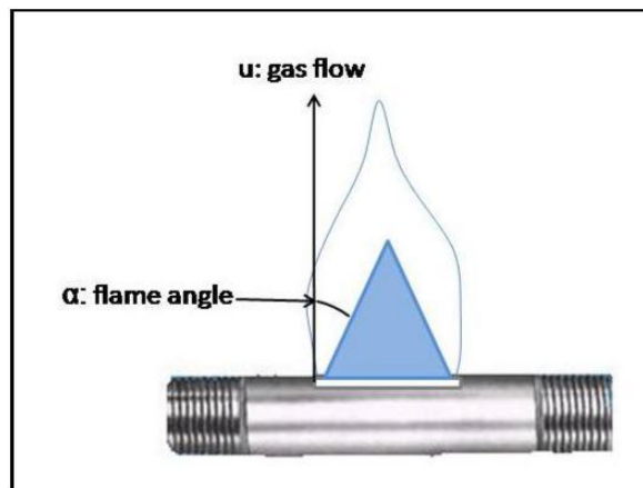
Figure 2: Illustration of Experimental Parameters used to calculate Burning Velocity
