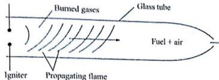
Flame propagation in a tube containing flammable fuel-air mixture.
