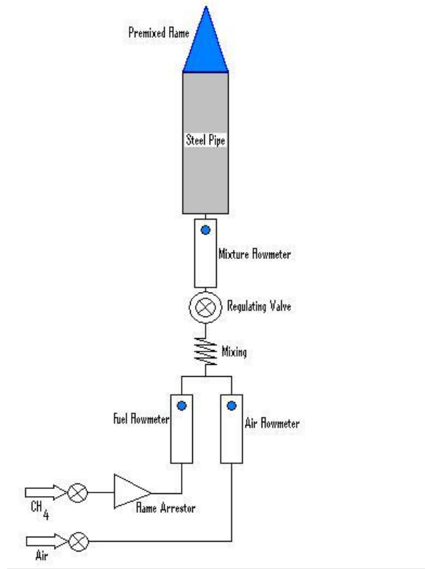
Figure 4: Typical Bunsen Burner
