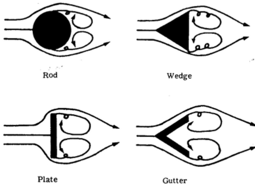
Figure 8.31 Flame stabilization by recirculation
