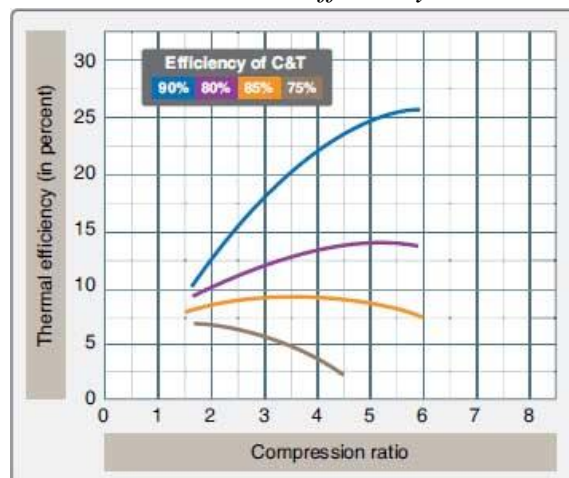
Fig. 2. Turbine and compressor efficiency vs. thermal efficiency.
