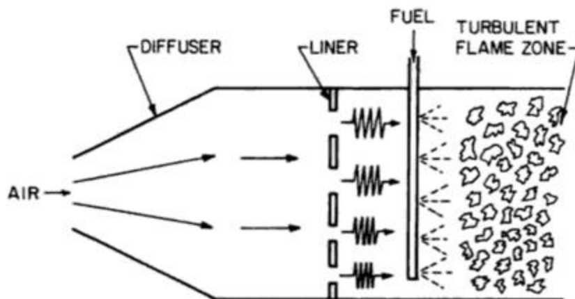
Burning velocity model for combustion efficiency
