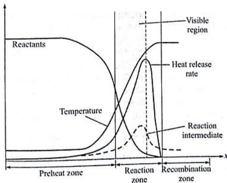
The structure of one-dimensional laminar premixed flame.
