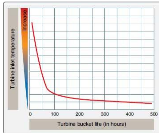
Fig.3. Effect of turbine inlet temperature on turbine bucket life.
