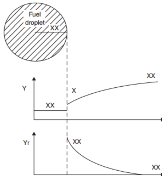
Fig. Quasi-steady evaporation model for a droplet in a static gas without combustion.
