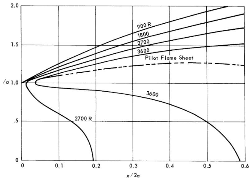
Isotherms and pilot flame sheet.
