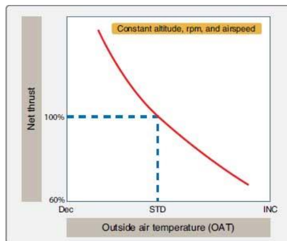
fig.4. Effect of OAT on thrust output.
