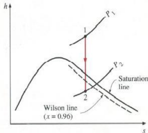
The h - s diagram for the isentropic expansion of steam in a nozzle.
