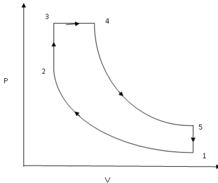
Fig.6: P-V Diagram of Dual Cycle.
