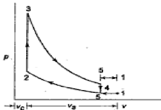
Theoretical p-v diagram for two-stroke petrol engine v_c -clearance volume v_s -stroke volume 1-5 piston travel during open period
