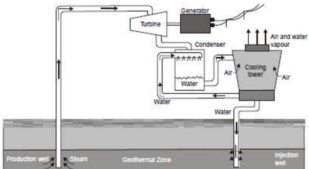
Fig. 2.34. Schematic of the Dry Steam Power Plant.
