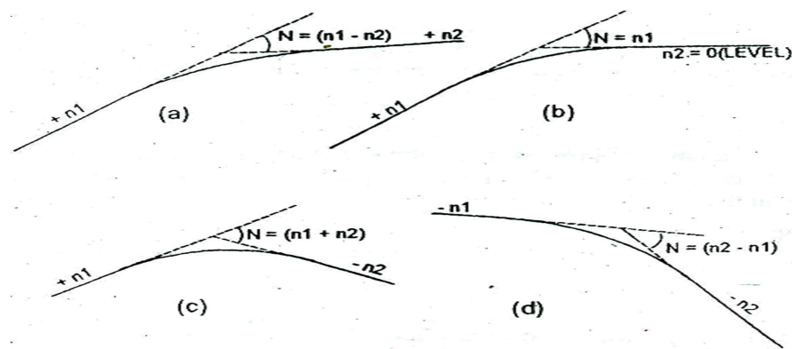
Fig. 4.34 Types of summit curves
