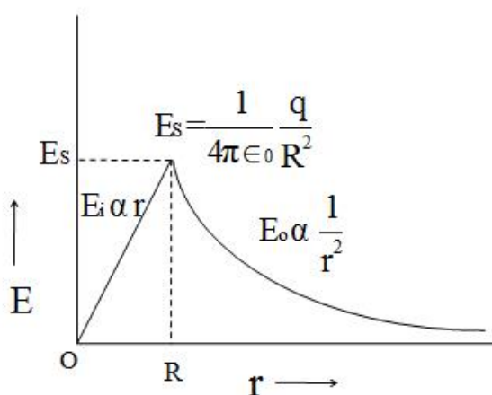
Figure 3B.4 Electric field due to a uniformly charged sphere as a function of distance from the centre of sphere.
