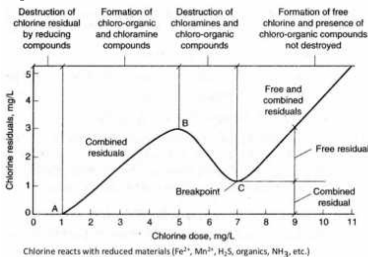
Breakpoint Chlorination
