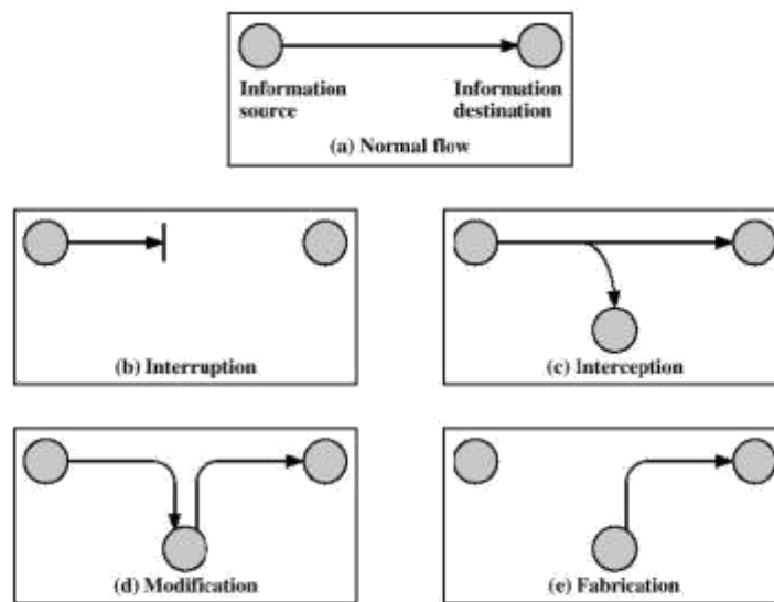
Figure 1.1 Security Threats
