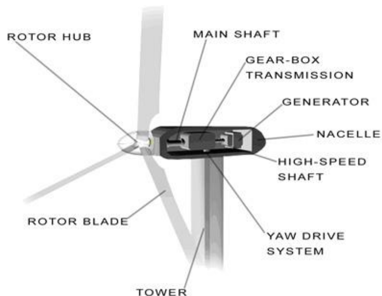
Fig. 1.9 Wind mill
