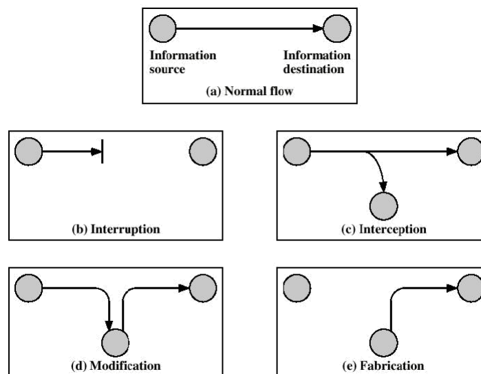
Figure 1.1 Security Threats
