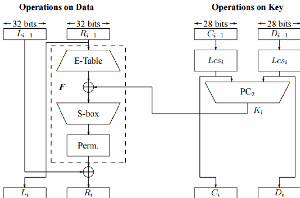
Figure 10.1 : Details of a single DES round.
