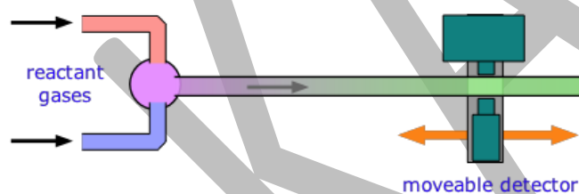
A continuous flow fast kinetic system.
