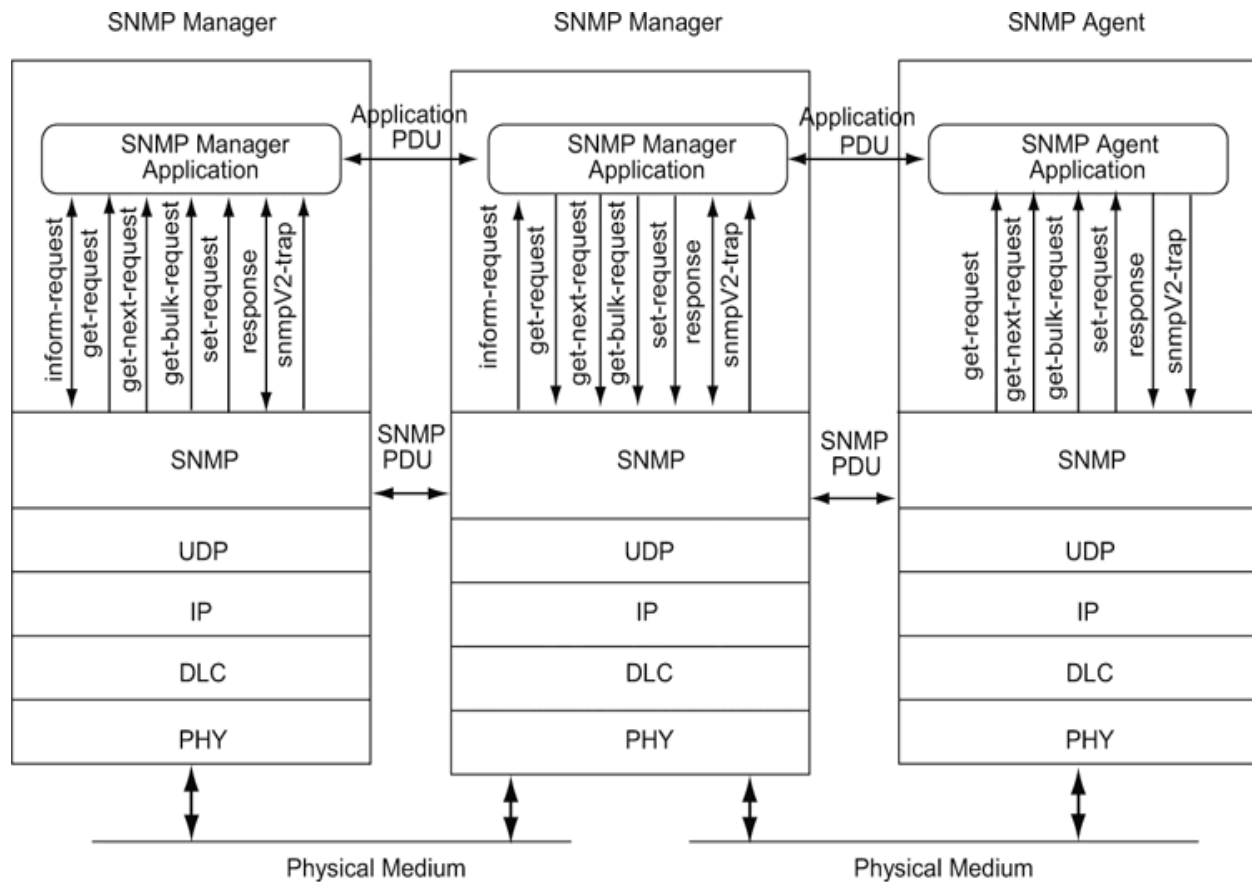
Figure SNMPv2 Network Management Architecture
