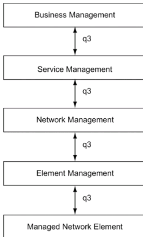
Figure TMN Service Architecture
