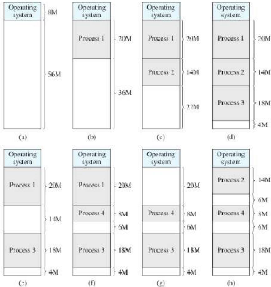
Fig.3.9. The Effect of dynamic partitioning
