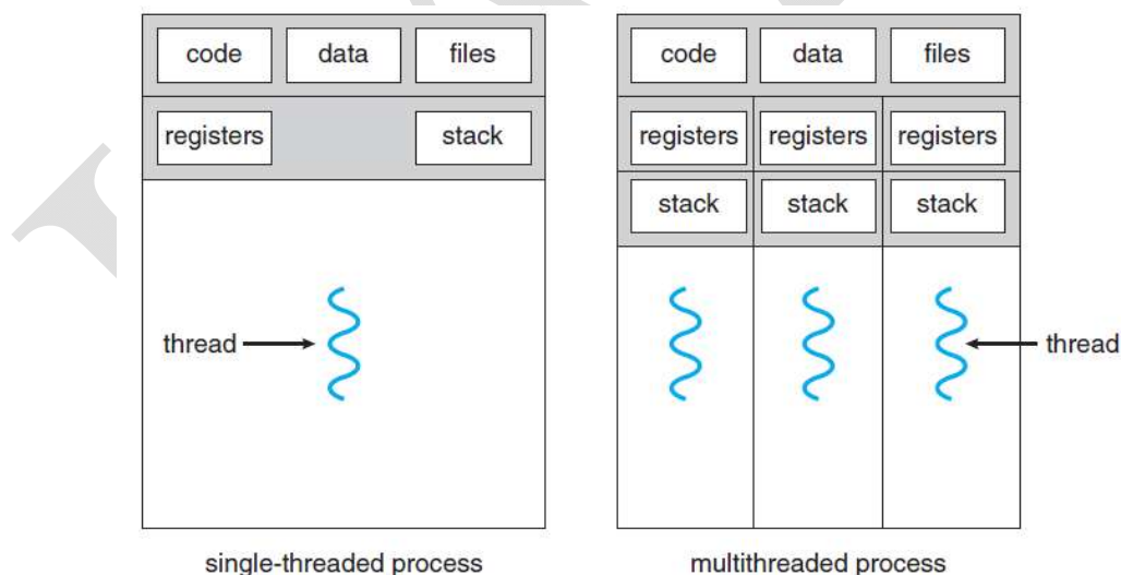
Fig 2.6. Single-threaded and multithreaded processes
