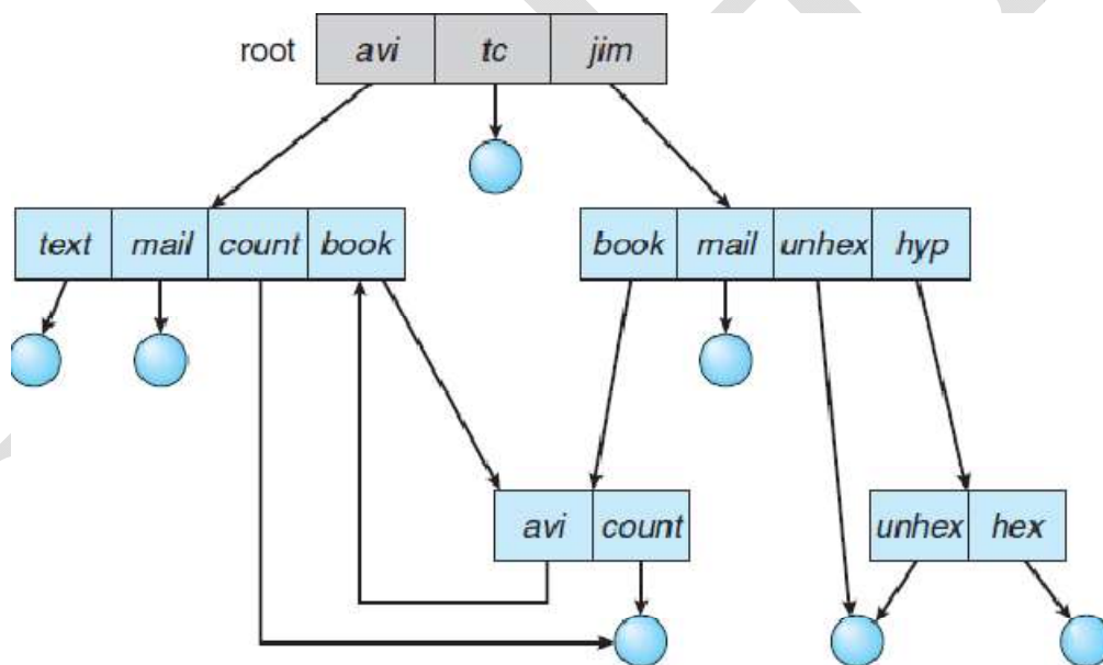
Fig 4.5.General graph directory.
