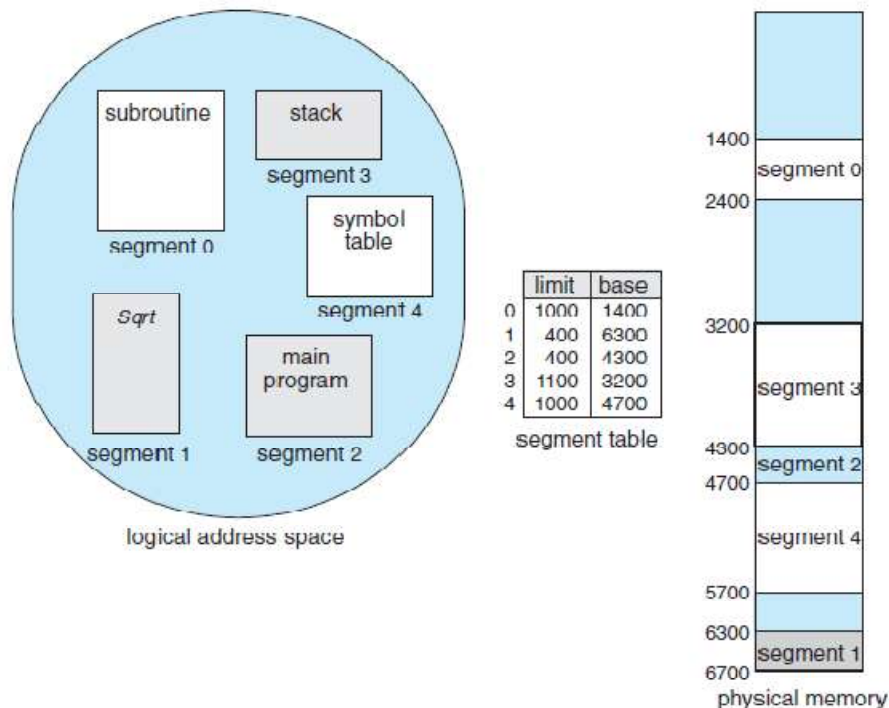
Fig 3.13. Segmentation
