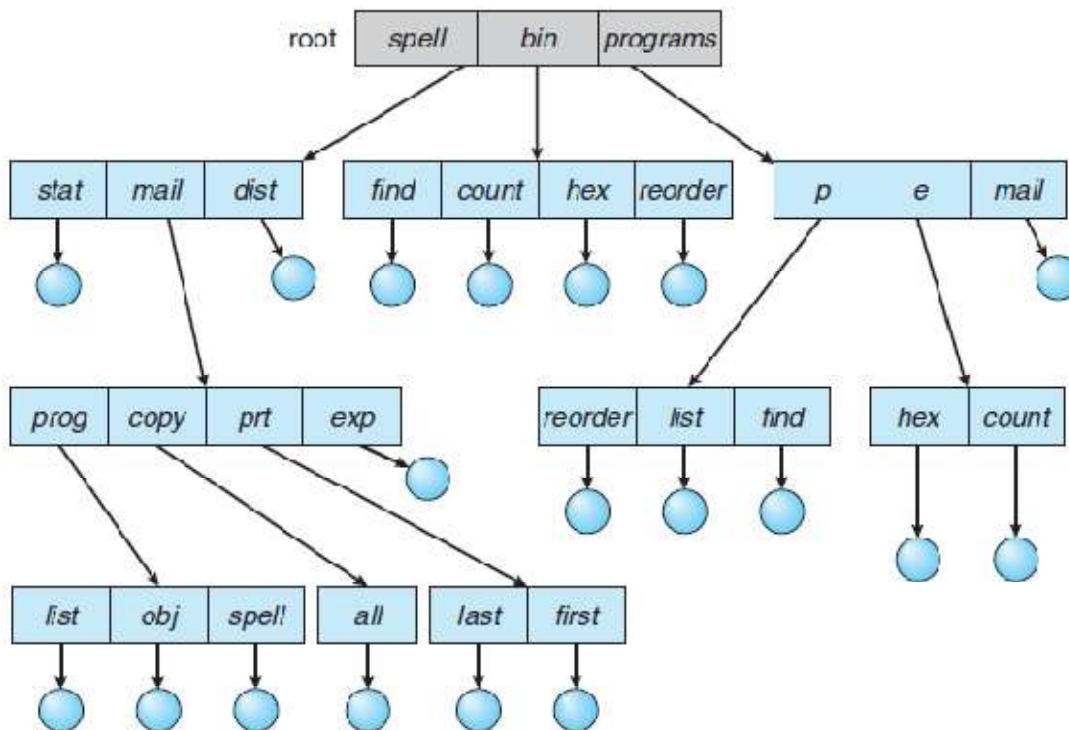
Fig 4.3.Tree-structured directory structure.
