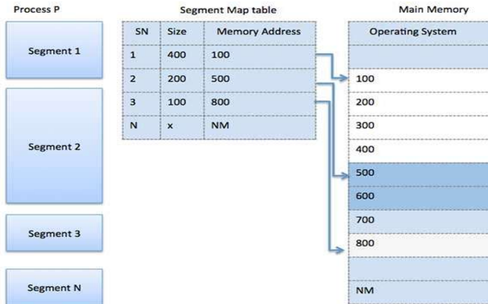
Fig 3.14. Segmentation Process
