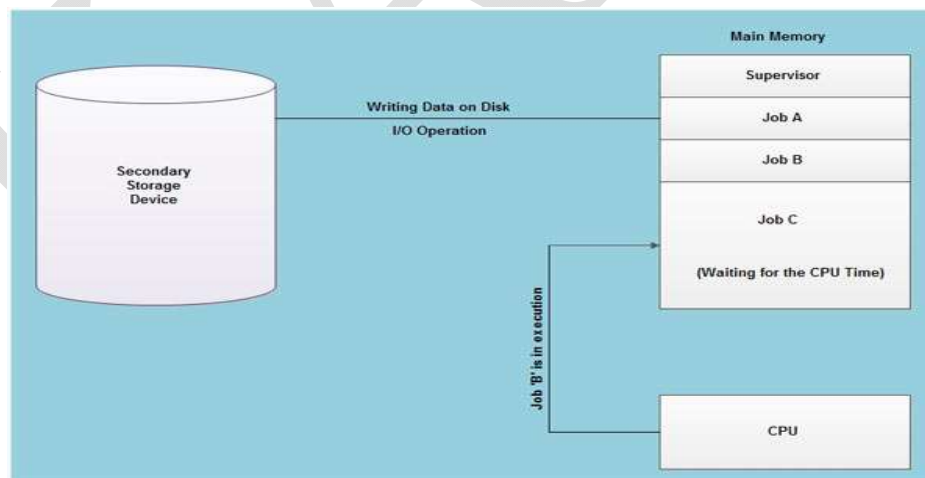
Figure 1.3. A simple process of multiprogramming.
