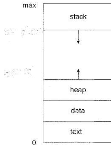
Process in memory
