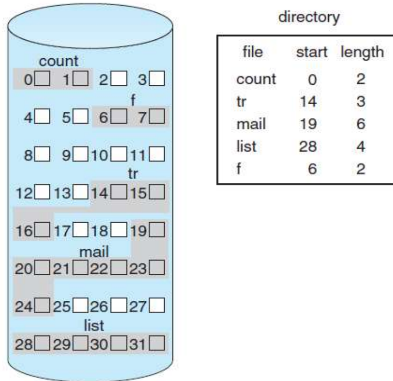
Fig 4.6. Contiguous allocation of disk space
