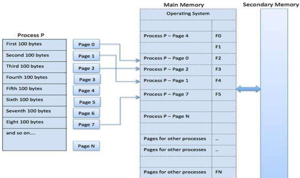
Fig 3.10. Paging Process
