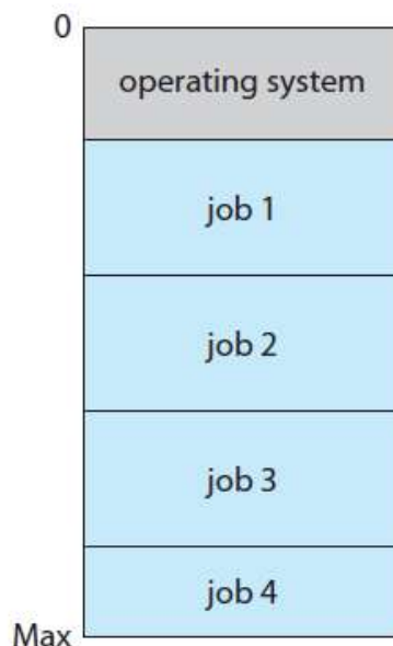
Figure 1.4 Memory layout for a multiprogramming system.
