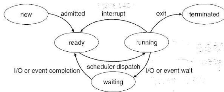
Fig 2.3 Diagram of process state
