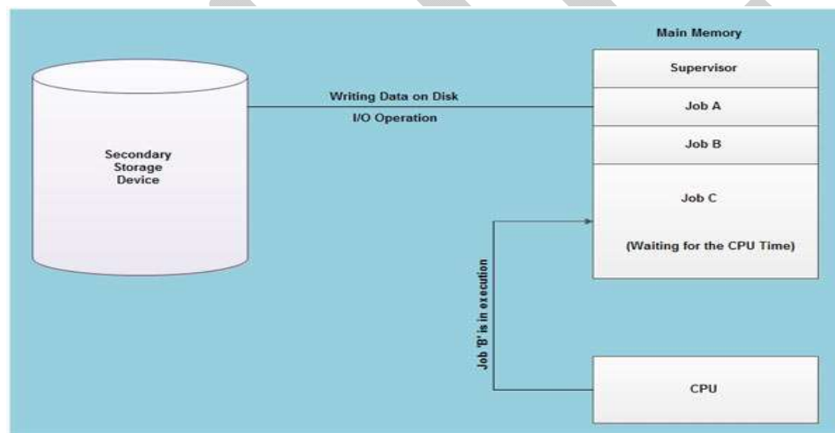
A simple process of multiprogramming.
