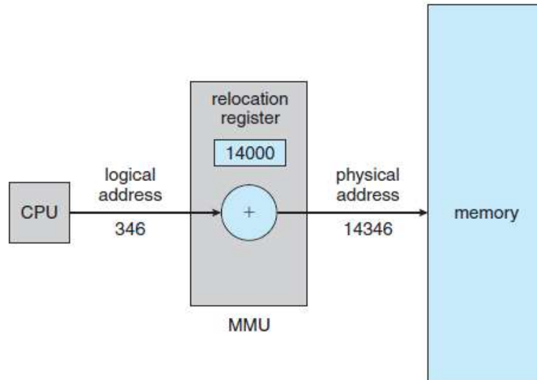
Fig 3.2. Physical address and Logical Address
