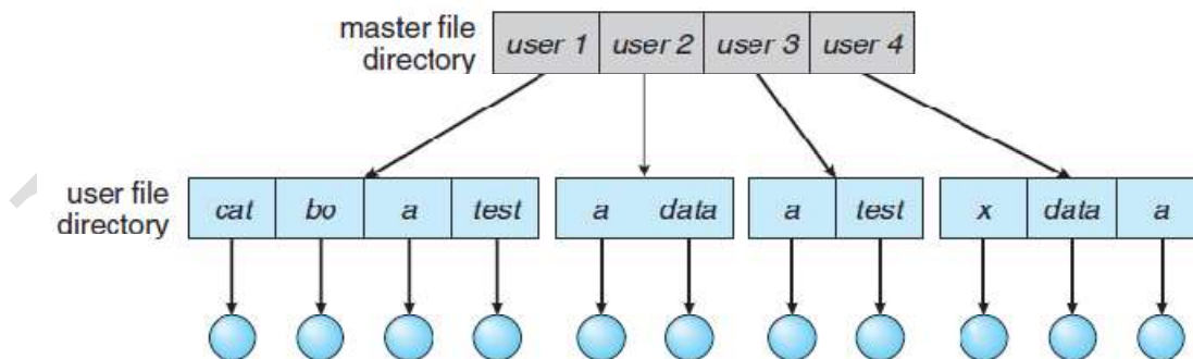
Fig 4.2. Two-level directory structure.
