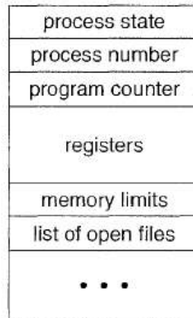
Fig 2.4. Process Control Block
