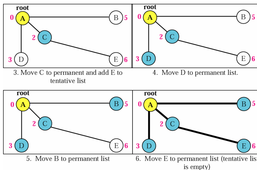
Example of formation of shortest path tree
