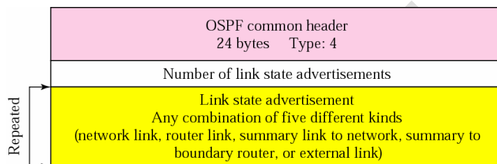
Link state update packet
