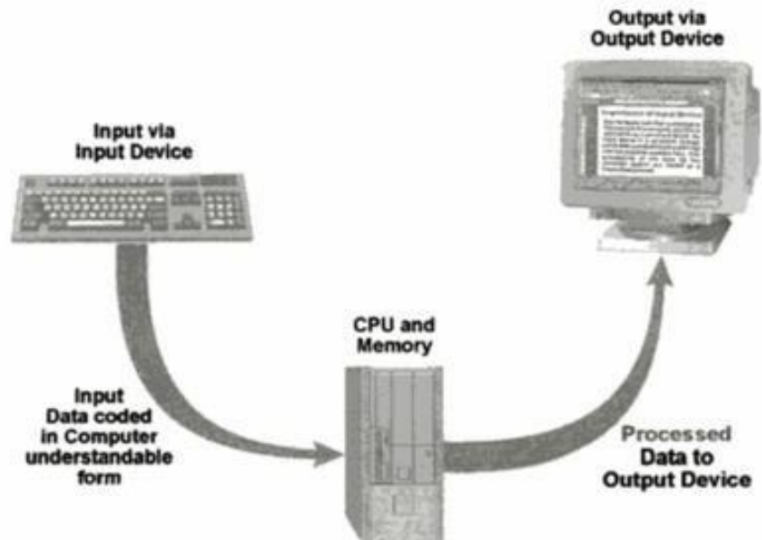
Figure 6.1 Data Processing
