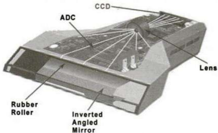
Figure 6.20 Inside Hand-Held Scanner
