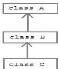
Multilevel inheritance
