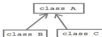
Heirarchical inheritance
